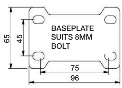
75 -125MM RIGID CASTOR
