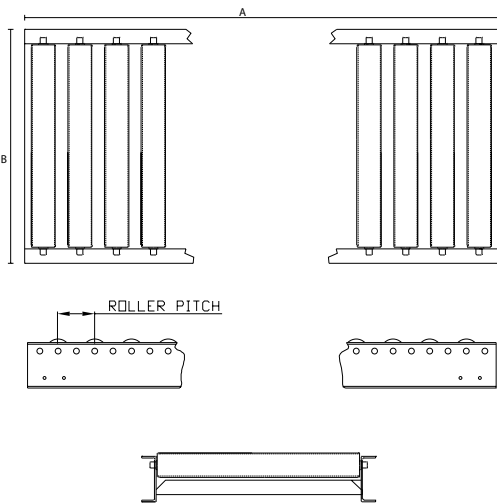
ROLLER SITS ABOVE CHANNEL STEEL ROLLER 50MM DIAMETER NYLON ROLLER 48MM DIAMETER
