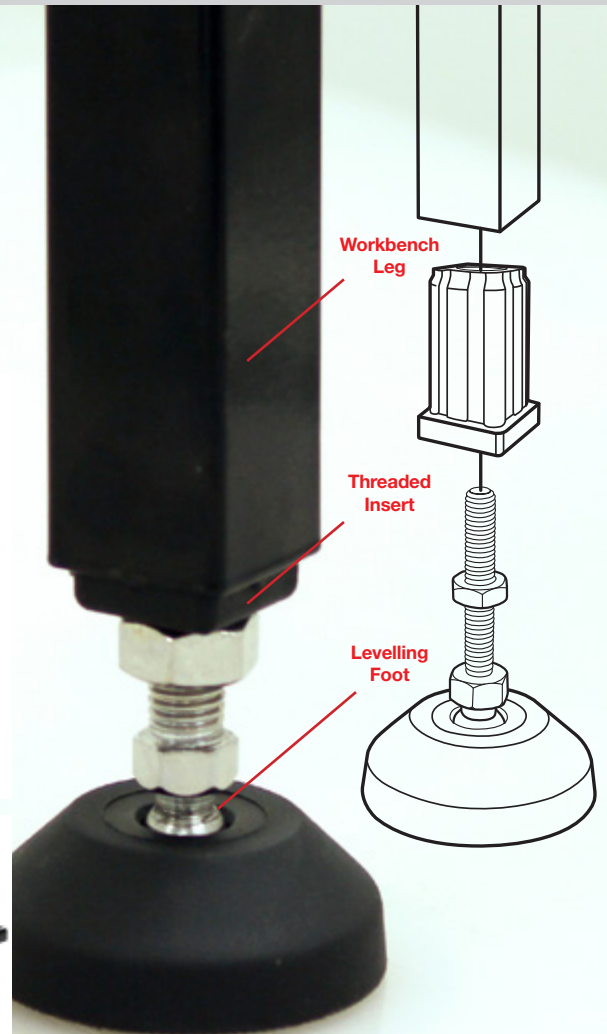
Bolt Down Levelling Foot
