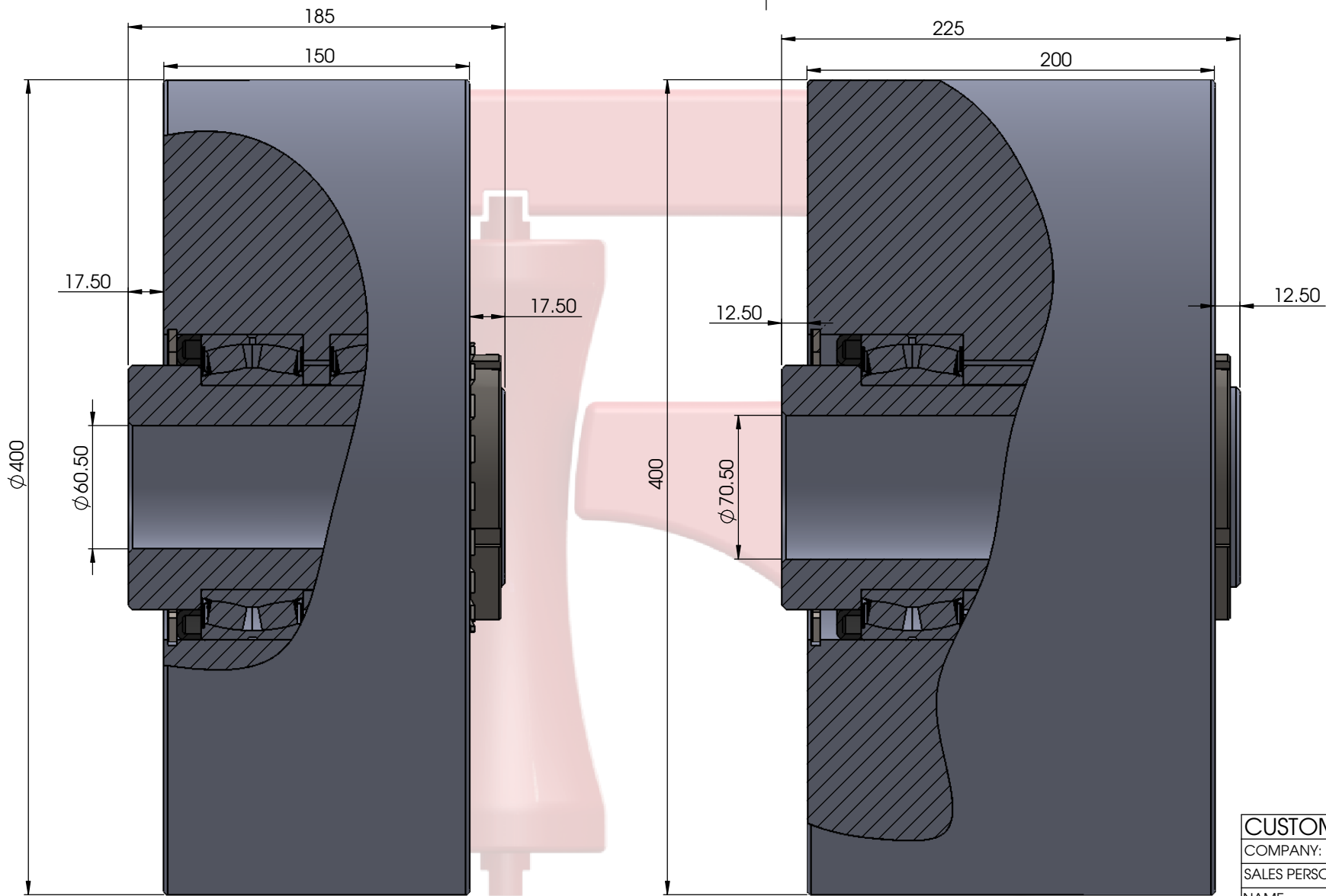
ST400X200 (100MM SPHERICAL ROLLER BEARINGS TO SUIT M60 PRECISION BOLT)
